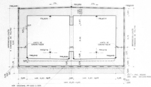
CORTE TRANSVERSAL 8-8
