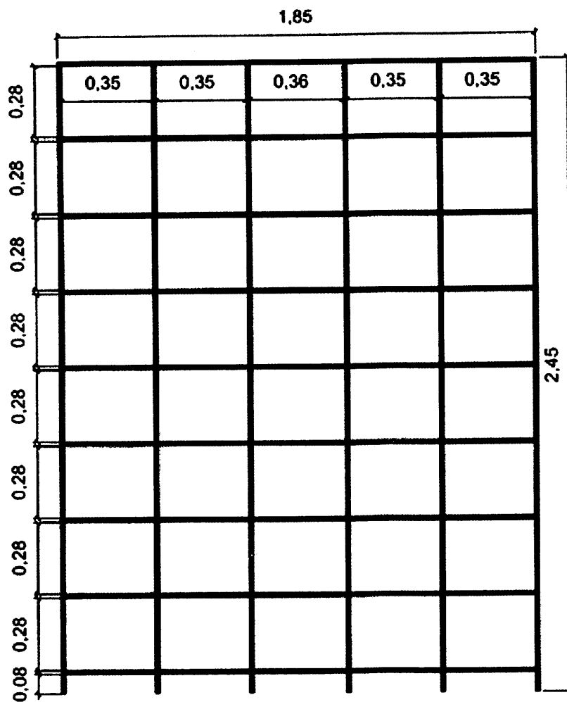
VISTA FRONTAL
